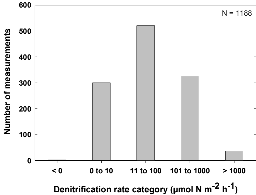
Figure 3. Frequency distribution of denitrification rates measured in estuaries.
